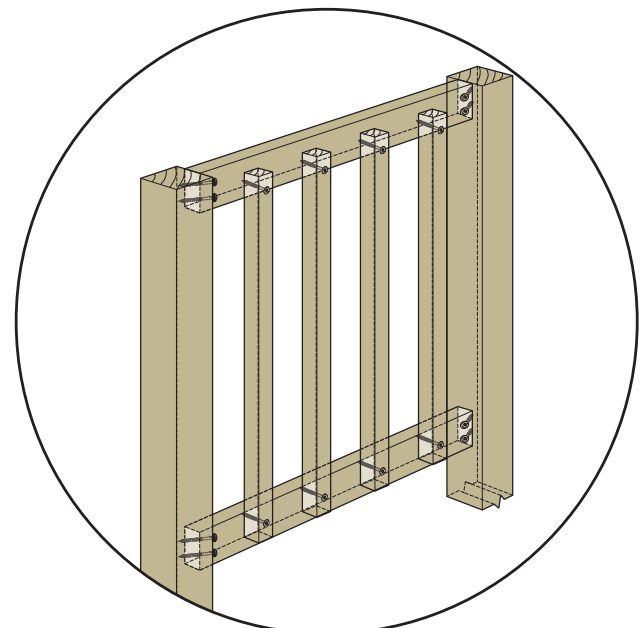
Baluster Perspective View
