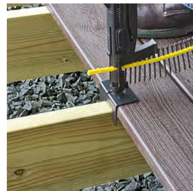
Shown with Deck Clip QDECKCLIP-RC
