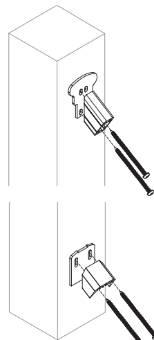
UPPER NEWEL POST (Figure 2.1)
